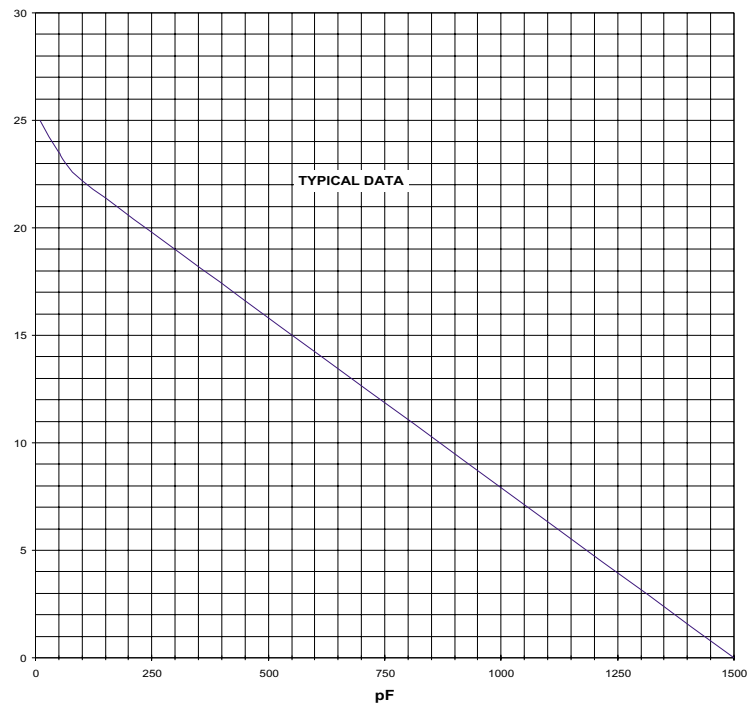
CAPACITANCE VS TURNS CVDP-1500
