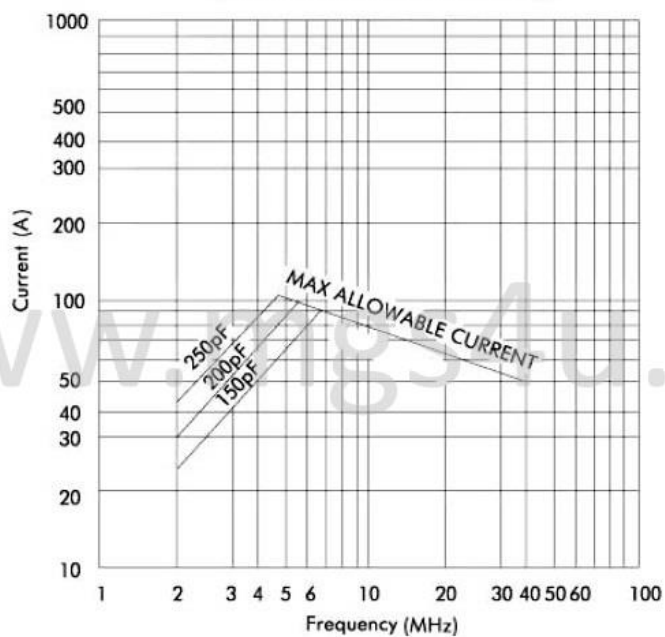
CKT250, 200, and 150 CONTINUOUS RMS AMPERES vs. FREQUENCY (at 20kV PEAK WORKING VOLTAGE)
