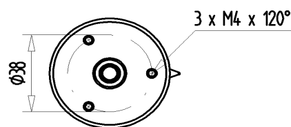
VIEW X
