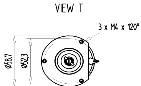
VIEW B
