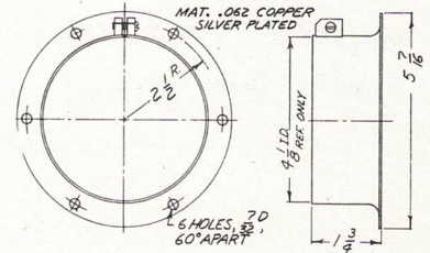
FM4 Flange Mount
