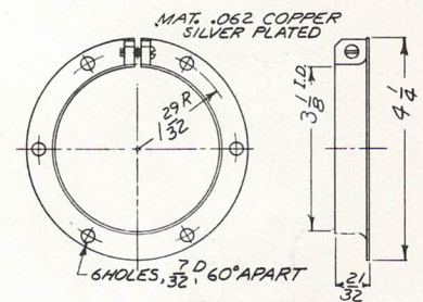
FM3C Flange Mount
